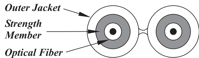
Figure 2—Fiber optic cable is available as paired cable (duplex cable) with an appearance similar to “zip cord.”
